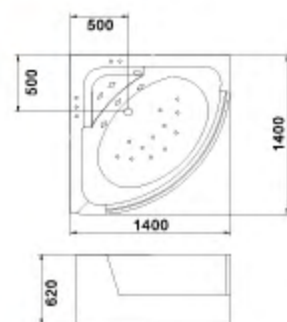
C-474 Size:1400x1400x620/mm
