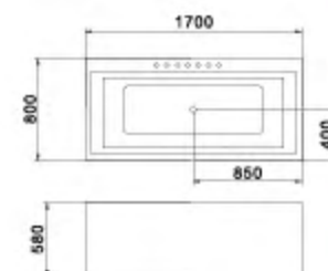
C-476 Size:800x1700x580/mm
