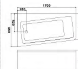
C-463-XH(L) Size:950X1700X580/mm
