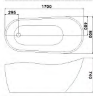
C-3213 Size:800X1700X740/mm
