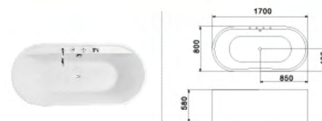
C-3229 Size:800X1700X580/mm
