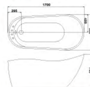
C-3214 Size:800X1700X740/mm
