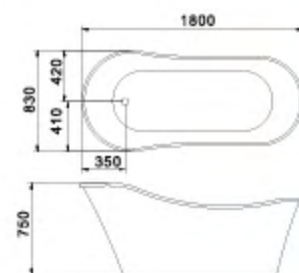
C-3228 Size:830X1800X750/mm
